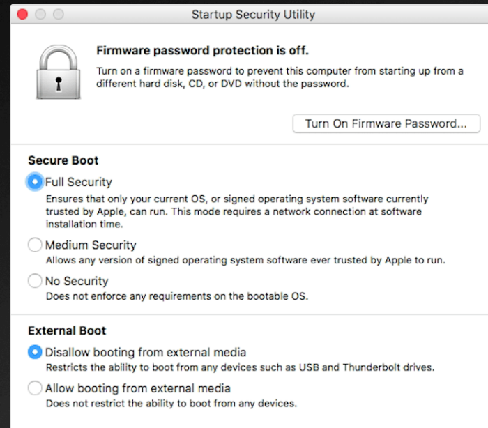
Startup Security Menu - Intel T2 Macs
